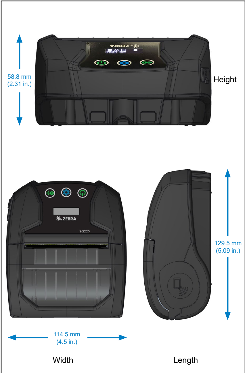
Figure 22 • Printer Dimensions
