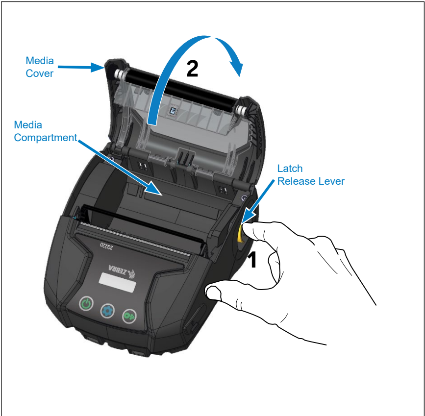
Figure 3 • Opening the Printer
